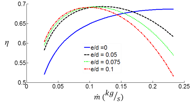
Figure 1. Overall efficiency of the solar air heater in smooth and ribbed surface as a function of rib height and air mass flow rate
