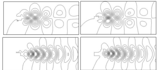
Figure 2. Four strongest modes of pressure field
