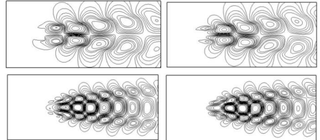
Figure 1. Four strongest modes of streamwise velocity component
