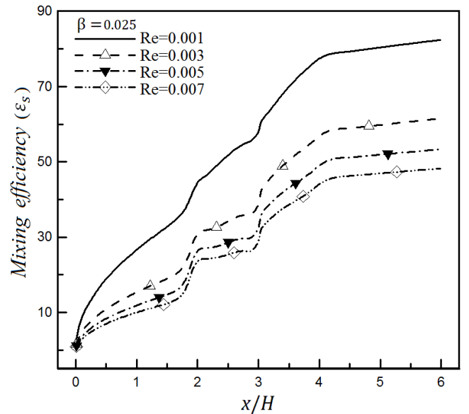
Figure 3. Mixing efficiency changes per specific slip coefficient (0.025) and different Reynolds number for (np-pn) pattern
