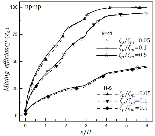
Figure 2. Mixing efficiency value of Nernst–Planck model and H-S model for K=41
