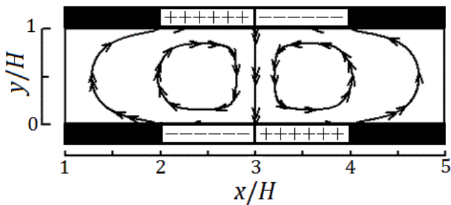
Figure 1. Schematic of electro-osmotic streamline for a prescribed configuration of patches in middle section
