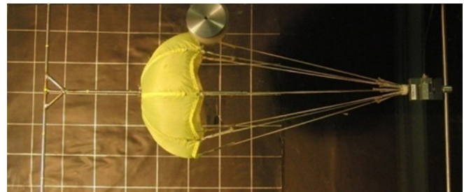
Figure 1. Test set up
