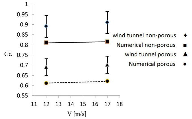
Figure 4. Drag coefficients
