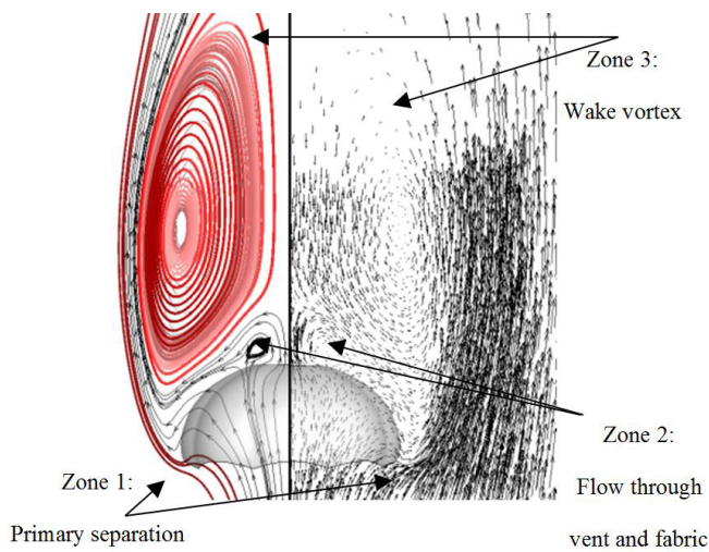
Figure 3. Surface streamlines and vectors around 3D parachute
