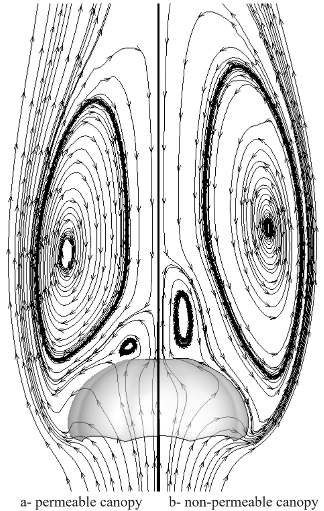
Figure 5. Comparison between canopies
