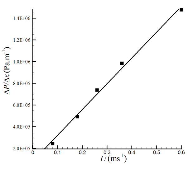
Figure 2. Results of the permeability test
