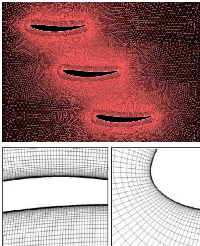
Figure 2. Grid domain near the blade surfaces
