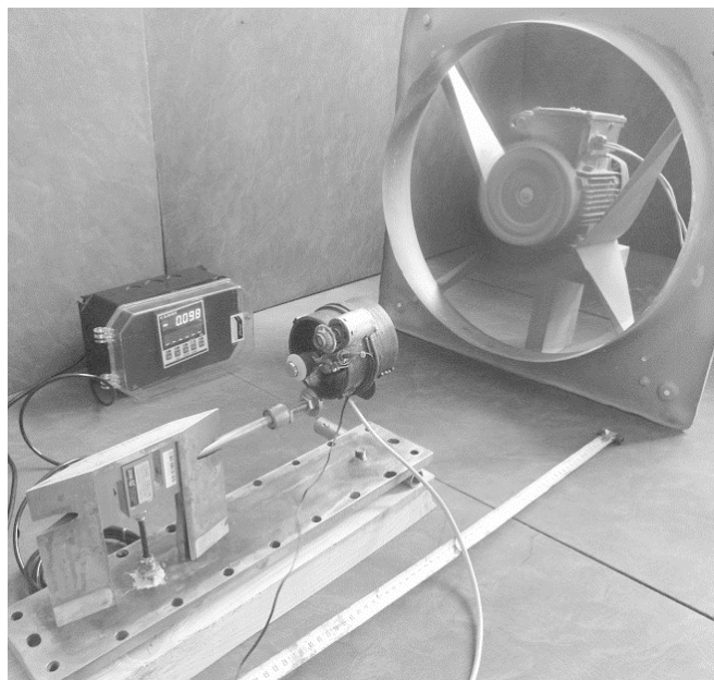
Figure 1. Experimental setup for test of the wind turbine in the wind flow
