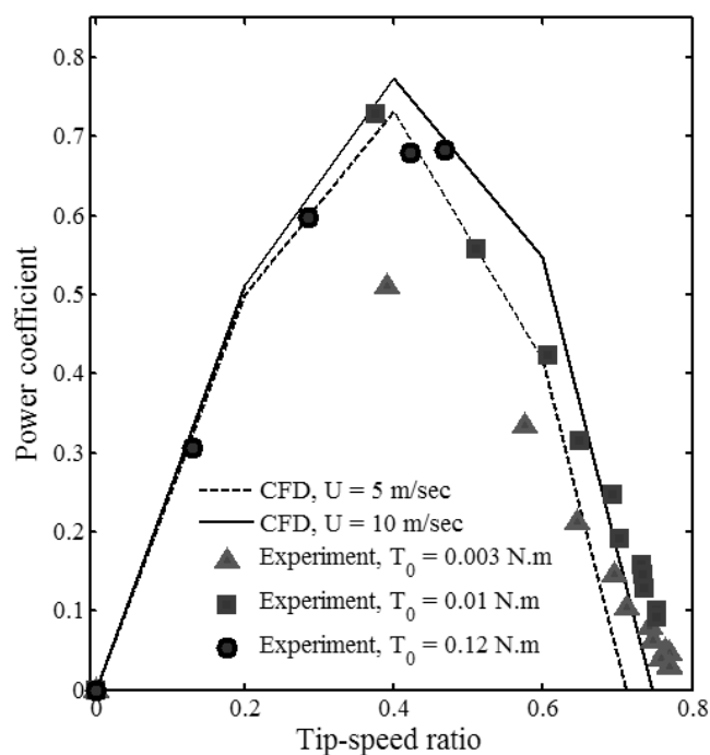
Figure 2. Experimental and numerical data for power-coefficient of wind turbine against tip-speed ratio
