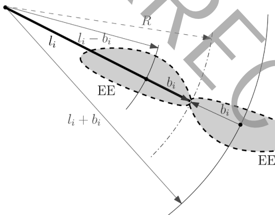
Fig. 2. The workspace of each taut cable
