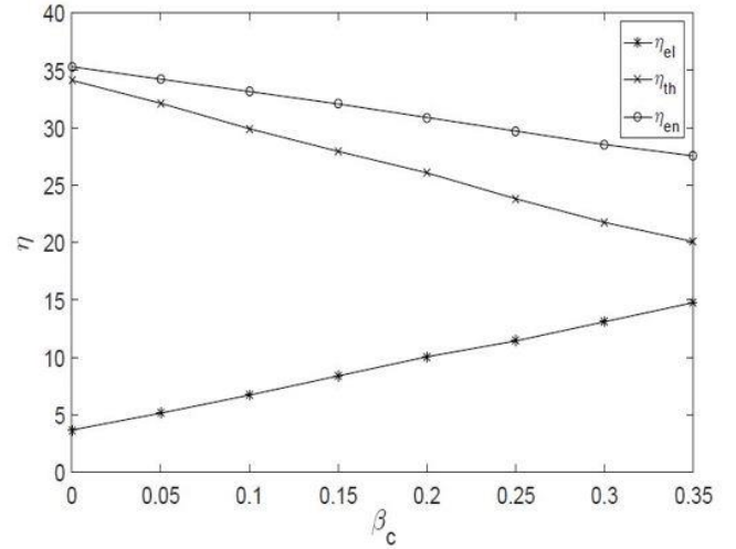
Fig. 2: Efficiency of the system in terms of the percentage of coating of the surface of the glass cover by photovoltaic cells
