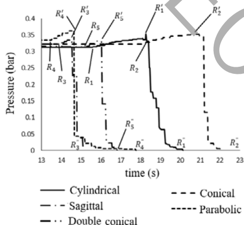
Fig. 2. Variation of the oil pressure for different cushions.
