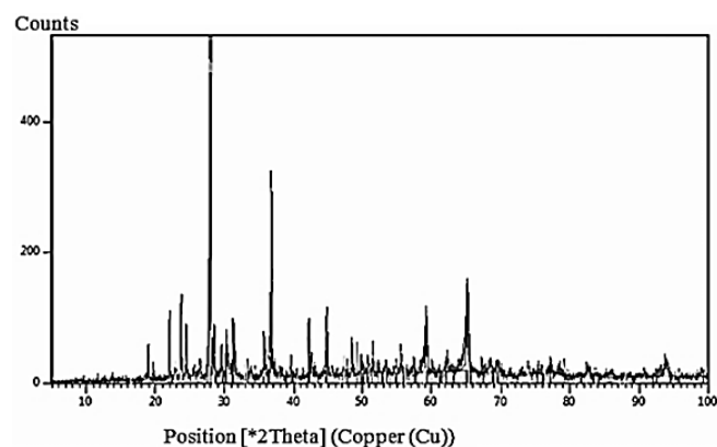
Fig. 1: XRD Spectrometric characteristics of ash on superheat pipes
