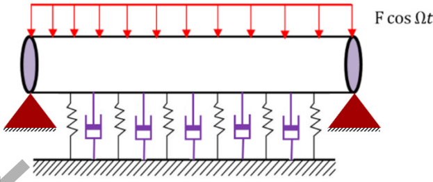
Fig. 1. Schematic of carbon nanotube under viscoelastic foundation
