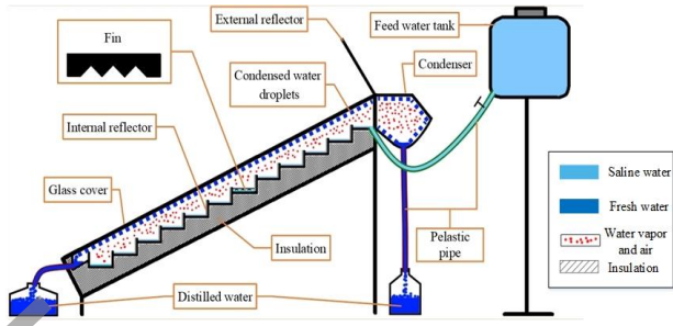
Fig. 1. Total schematic of cascade solar water desalination with fin, condenser, internal and external reflector
