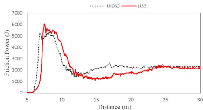
Fig. 6. Frictional power for different profile (UIC60 and U33)
