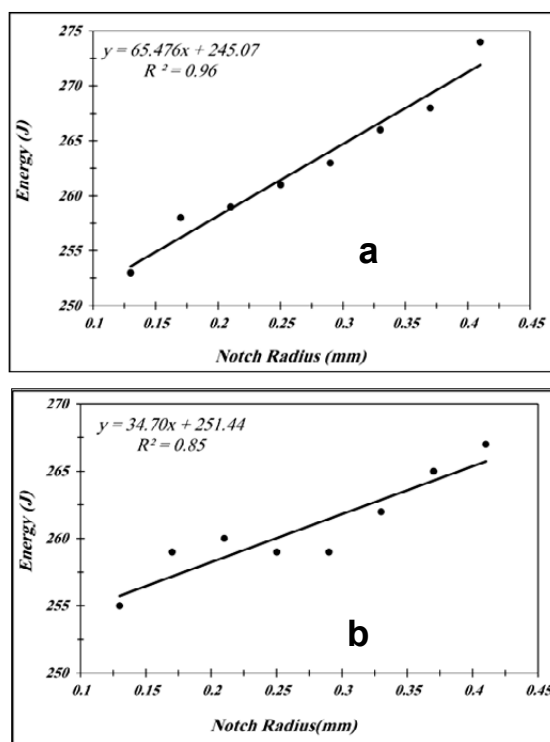
Fig. 2: Energy changes of the Charpy impact in terms of notch radius a) results of the simulation test b) results of the experiment
