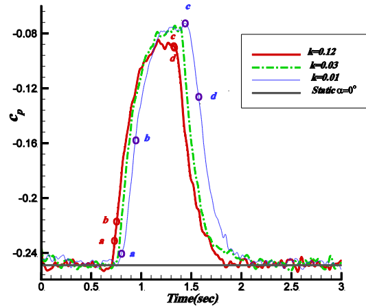
Fig. 2. Effect of reduced frequency on pressure distribution of x/c=0.53 at the lower surface, stop angle= 5^\circ
