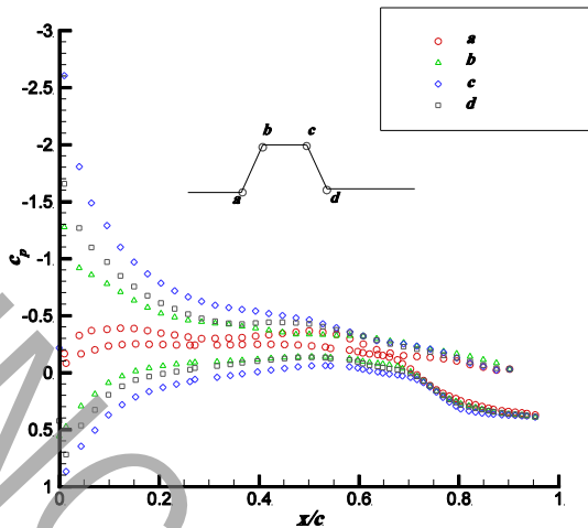
Fig. 1. Pressure distribution in four phases of the motion, k=0.01
