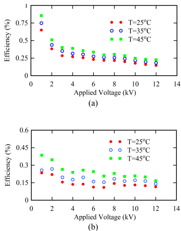
Fig. 1. Efficiency variations with applied voltage for film thickness : (a) n-hexane, (b) n-decane
