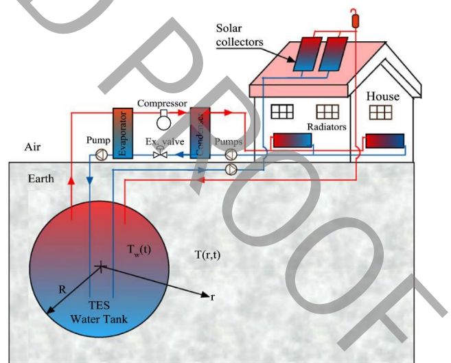
Fig. 1. Heating system by an underground source heat pump and photovoltaic thermal collectors [1]
