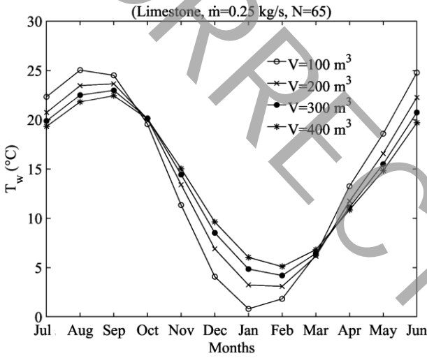
Fig. 3. Effect of changes in the volume of the water tank on the water temperature of the underground water tank
