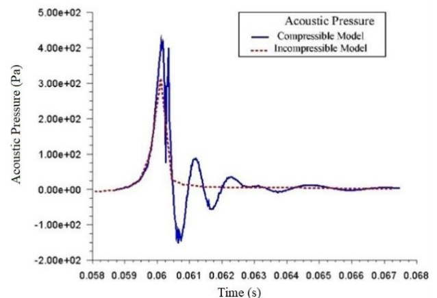
Fig. 3. Compressibility effect in the recording acoustic pressure
