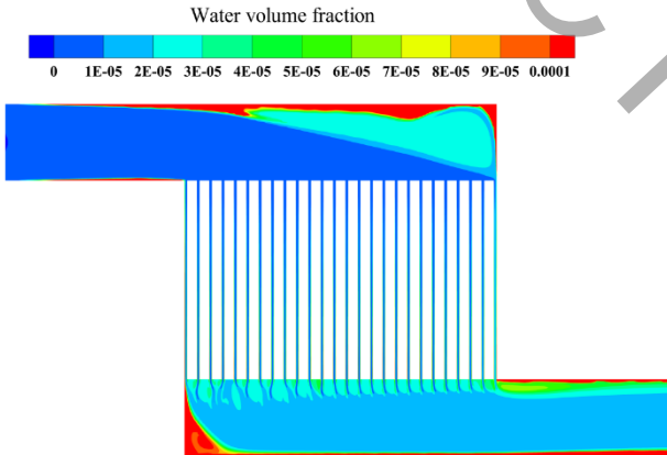
Fig. 2. Contours of liquid water volume fraction
