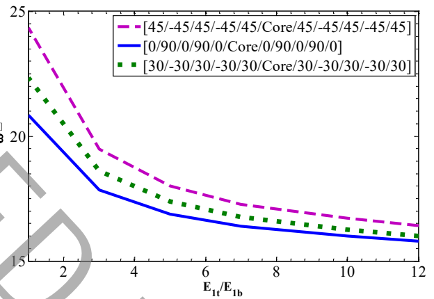
Figure 2. The effect of elastic modulus ratio of the face sheets on the dimensionless natural frequency
