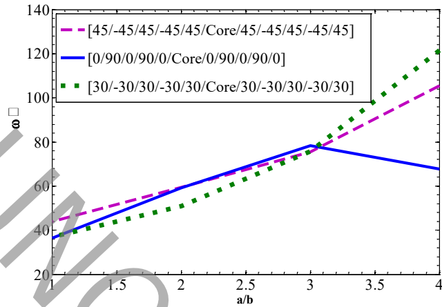
Fig. 3. The effect of panel length to width ratio on the dimensionless natural frequency
