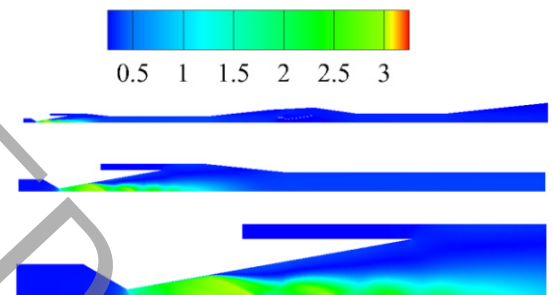
Fig. 4. Mach contour for engine ON and ejector OFF
