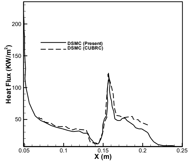
Fig. 4. Heat flux distribution on the double cones problem
