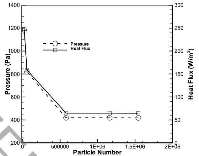
Fig. 5. Proper particle numbers for the double cones problem
