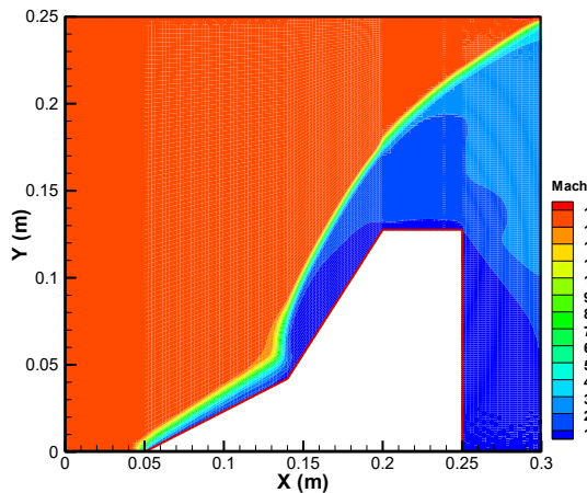
Fig. 3. Mach contours of double cones problem
