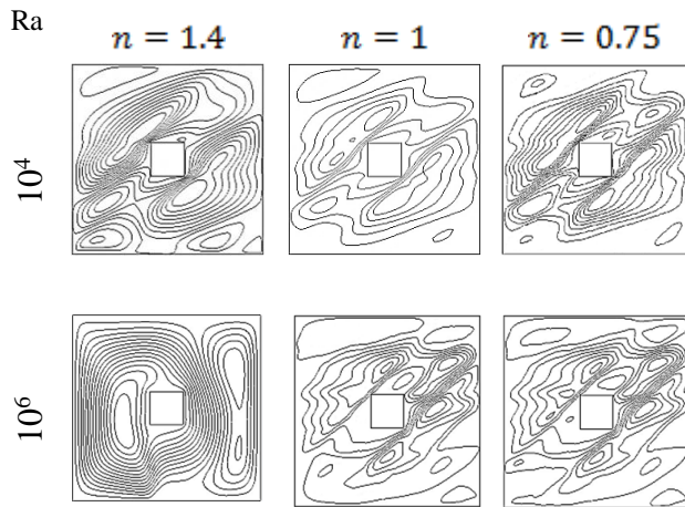
Figure 3. Flow lines in Rayleigh numbers and different indicators ( n ) in the presence of the magnetic field
