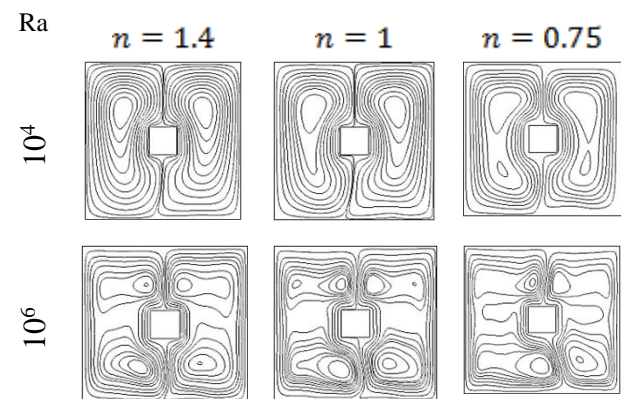
Figure 2. Flow lines in Rayleigh numbers and different indicators ( n )
