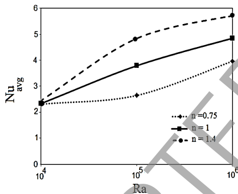
Figure 4. Variations of average Nusselt in the Rayleigh numbers for different power indexes
