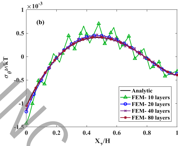
Fig. 3. Tangential stress distribution of hydrogel
