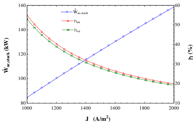
Fig. 2. Effects of current density on the power production and system energy as well as the exergy efficiencies
