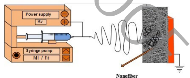
Fig. 1. A schematic of electrospinning setup
