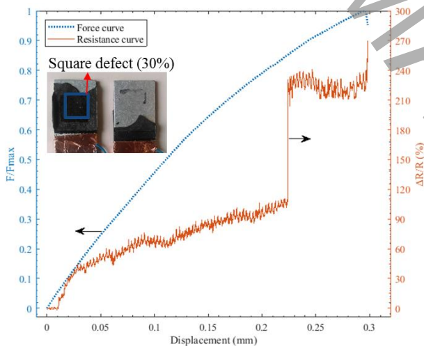
Fig. 4. Mechanical and electrical response of SLJ including 30% square defect area
