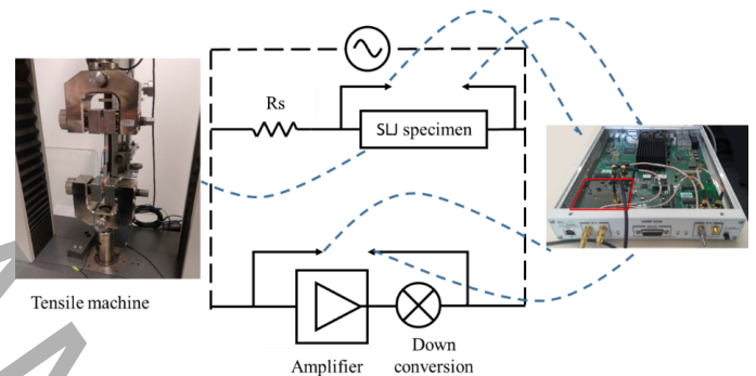
Fig 2. Electrical measurement setup during the tensile test.
