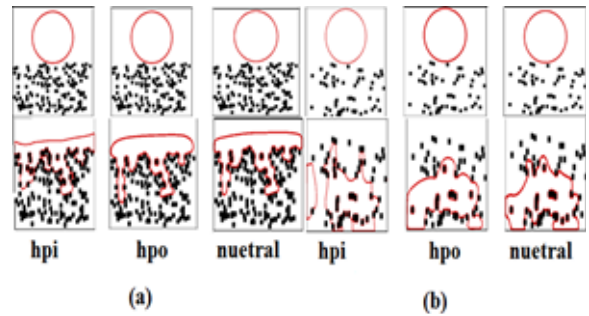
Figure 4. Pattern of penetration in three cases for (a) \epsilon=0/83 (b) \epsilon=0/93
