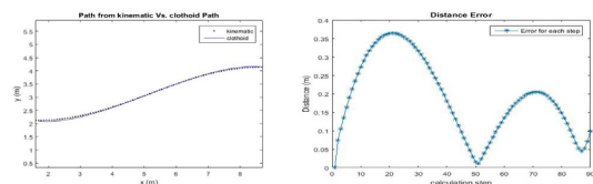
Fig.5. (a-left) Clothoid and cinematic paths. (b-right) Error value for each calculating step
