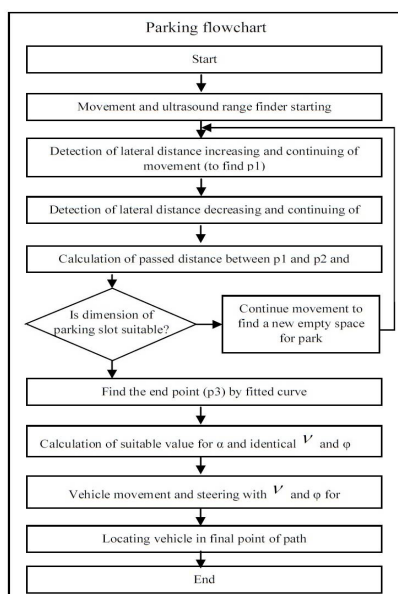
Fig.3. Parking flowchart with new algorithm
