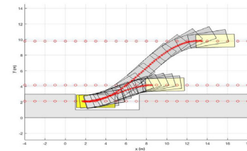
Fig.4. Parking manure with \sigma_{max} and \sigma_{max}/2
