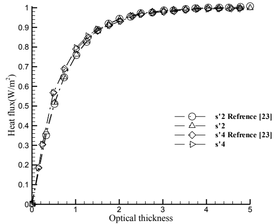
Fig. 3. Comparison of radiation fluxes of boundaries with reference [23] in term of gray radiation
