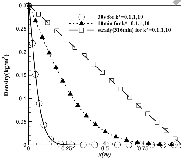
Fig. 9. Density changes based on location in a constant temperature of medium for three mass-absorption coefficients a) \kappa_a^* = 0.1 b) \kappa_a^* = 1.0 c) \kappa_a^* = 10.0
