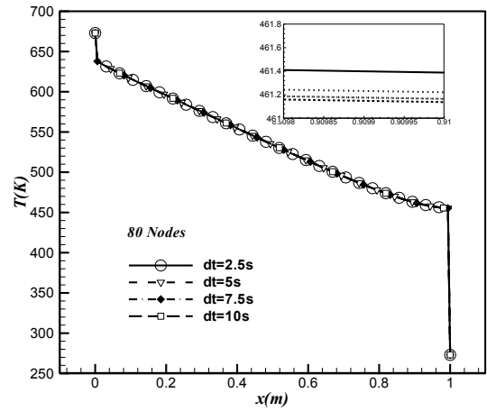
Fig. 5. Temperature distribution a) In a spatial network at different time b) At one time in different spatial networks
