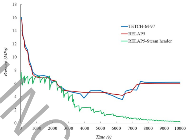
Fig. 8. The reactor outlet and steam header pressure during SB-LOCA with 25 mm break
