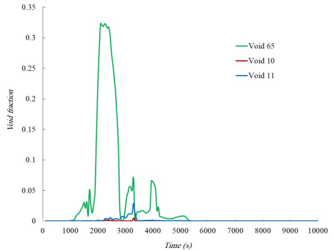
Fig. 9. Void fraction of reactor inlets (Vol. No.10 and 11) and upper plenum outlet (Vol. No. 65) during 25 mm break
