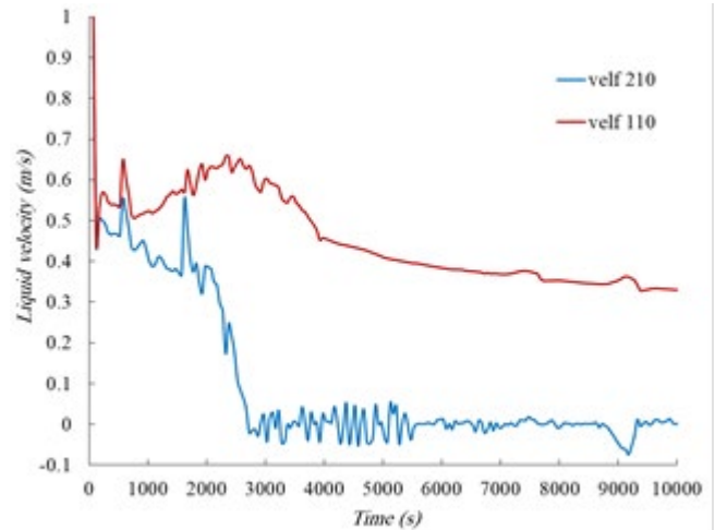
Fig. 11. Liquid velocity in the hot legs of first and second loops during SB-LOCA with 25 mm break
