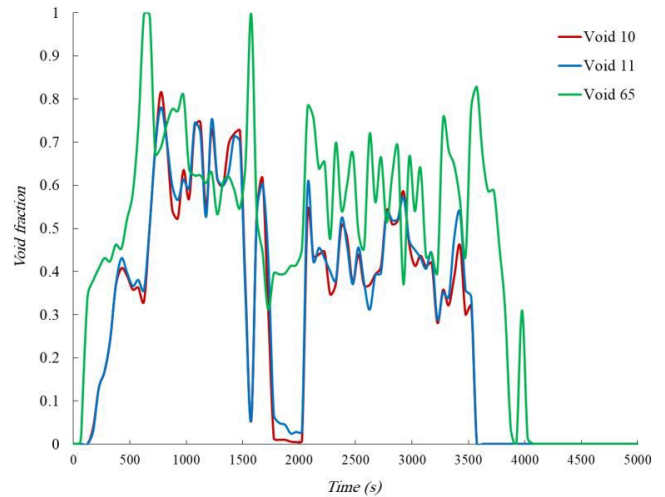
Fig. 5. Void fraction of reactor inlets (Vol. No.10 and 11) and upper plenum outlet (Vol. No. 65) during 100 mm break
