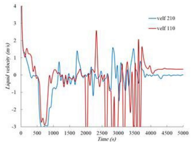
Fig. 7. Liquid velocity in the hot legs of first and second loops during SB-LOCA with 100 mm break
