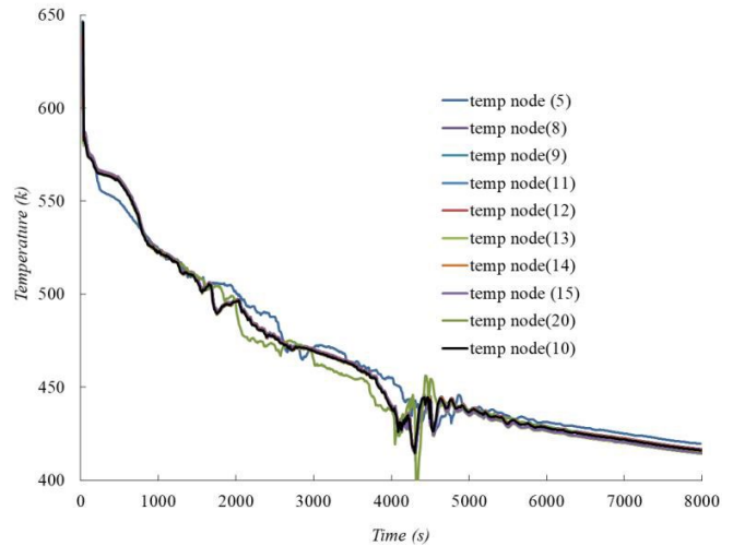
Fig. 3. Maximum clad temperature for different nodalization in the 100mm SB-LOCA
