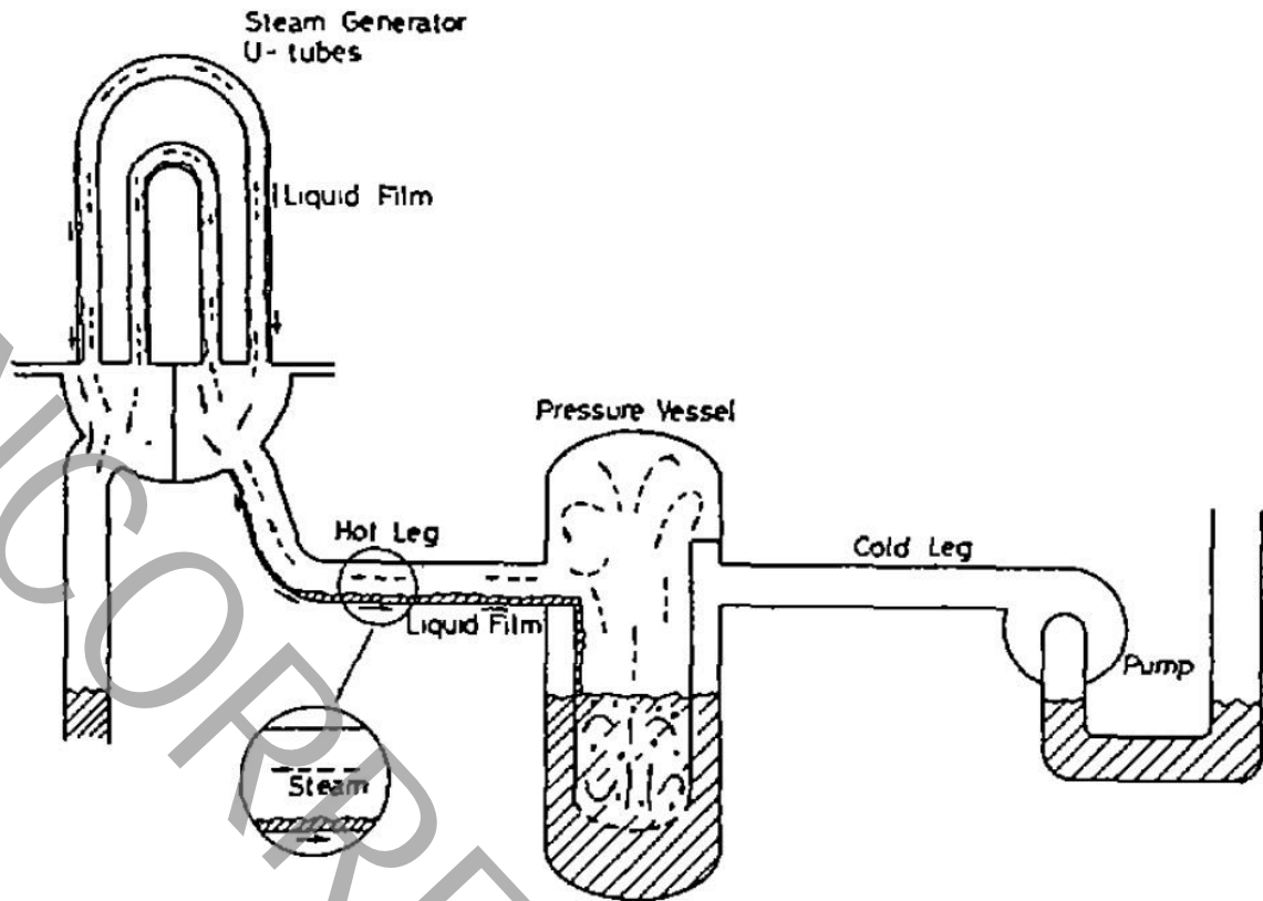
Fig. 1. Schematic of reflux condensation phenomena in the reactors with vertical steam generator [4]
