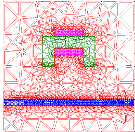
Fig. 2. Triangular elements
