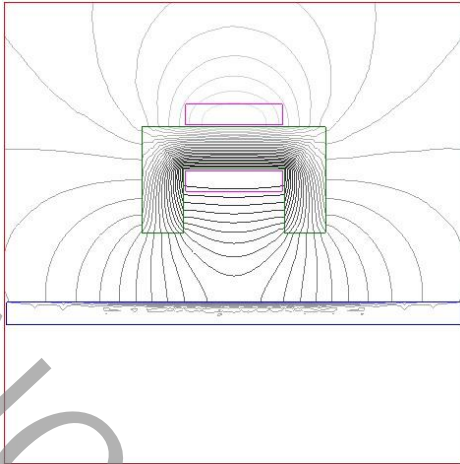
Fig. 4. Electromagnetic flux lines
