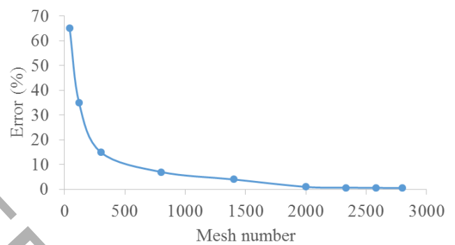
Fig. 3. Sensibility of analysis error to mesh size
