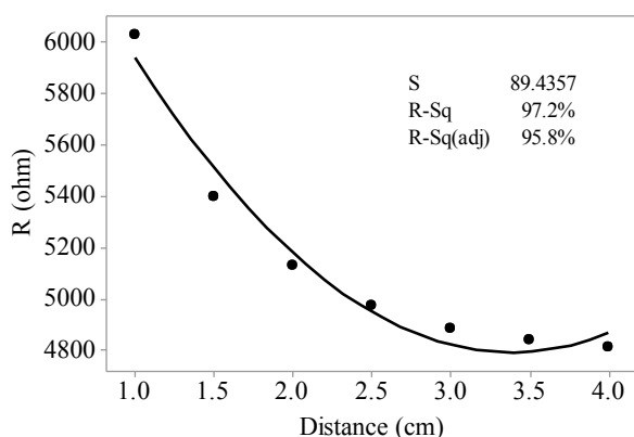
Fig. 10. Changes of ohmic resistance for different reinforcement cover in the frequency of 50 kHz
