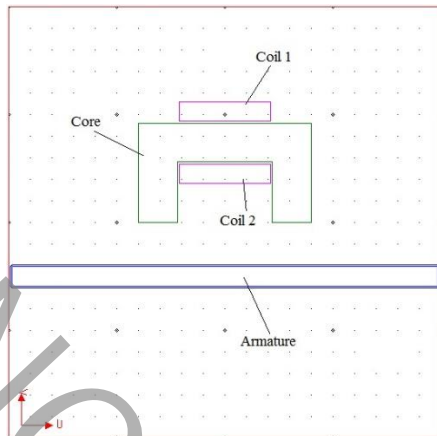
Fig. 1. 2-D simulation of the experiment geometry
