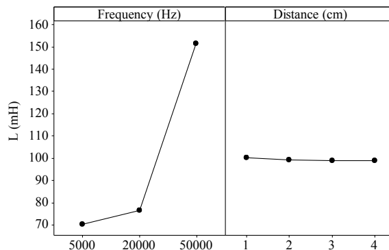
Fig. 8. Effects of the reinforcement cover and frequency on probe's inductance
