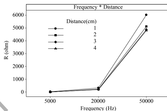
Fig. 9. Effects of the reinforcement cover and frequency on ohmic resistance of probe
