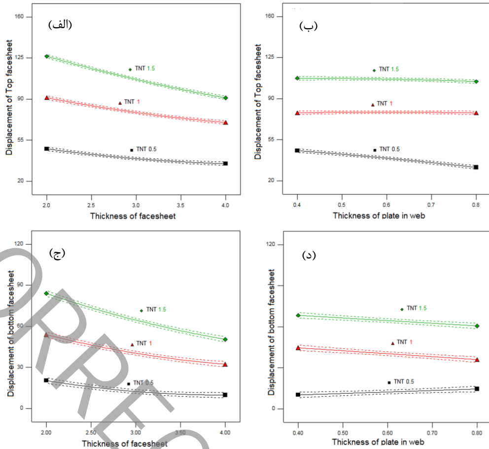
Fig. 7. The effect of the interaction of charge mass changes with the thickness of the metal plates (X1X4) and the thickness of the plates in the core (X3X4) on the displacement of the plates (a, b) top and (c, d) bottom
