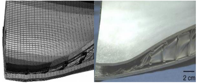
Fig. 3. Comparison between the results of experiments and simulated model
