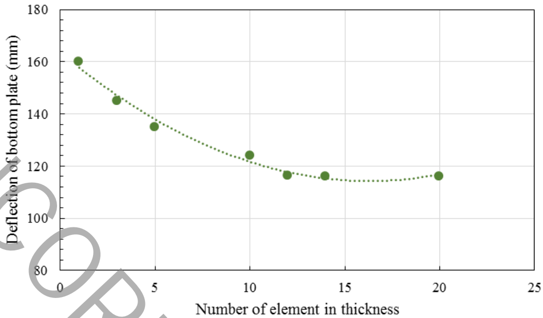
Fig. 2. Convergence of the results by changing the number of elements
