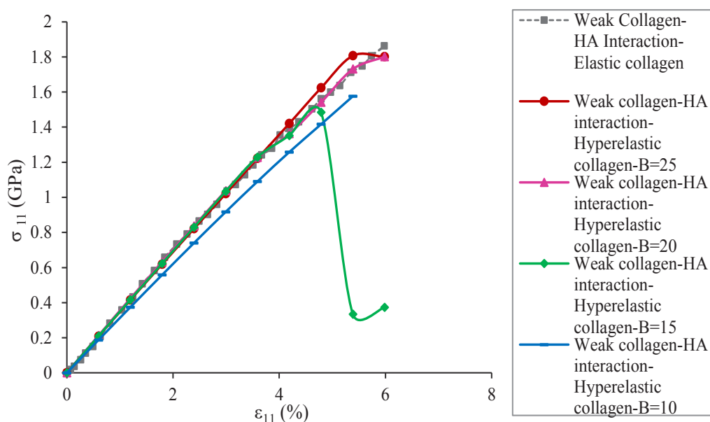
Fig. 19. Stress- strain results of mineralized collagen fibril with weak collagen- hydroxyapatite interaction with hyperelastic and elastic collagen properties with different B
