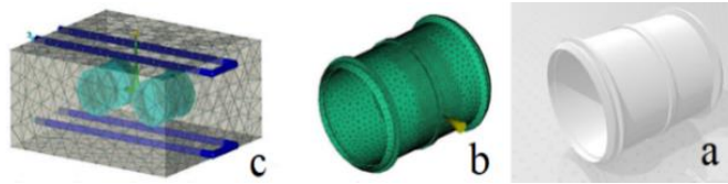
Fig1. a)part geometry b)meshed part c)mold geometry including runners and cooling channels
