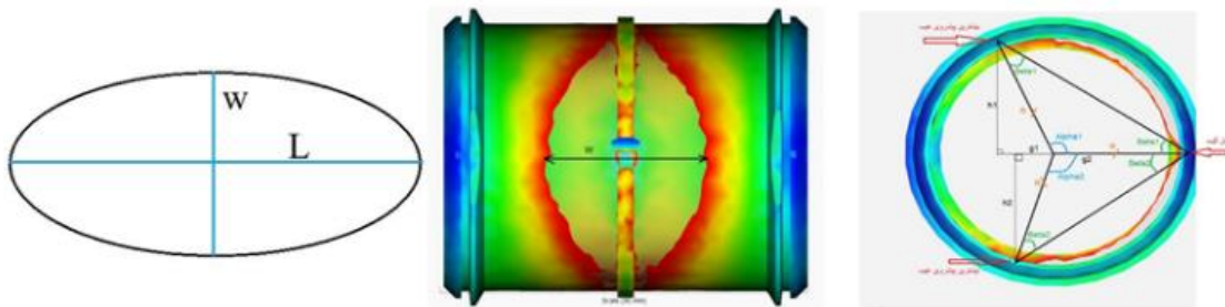
Fig2. Pictures of defect, showing W,L,Alpha1,Alpha2, and R
