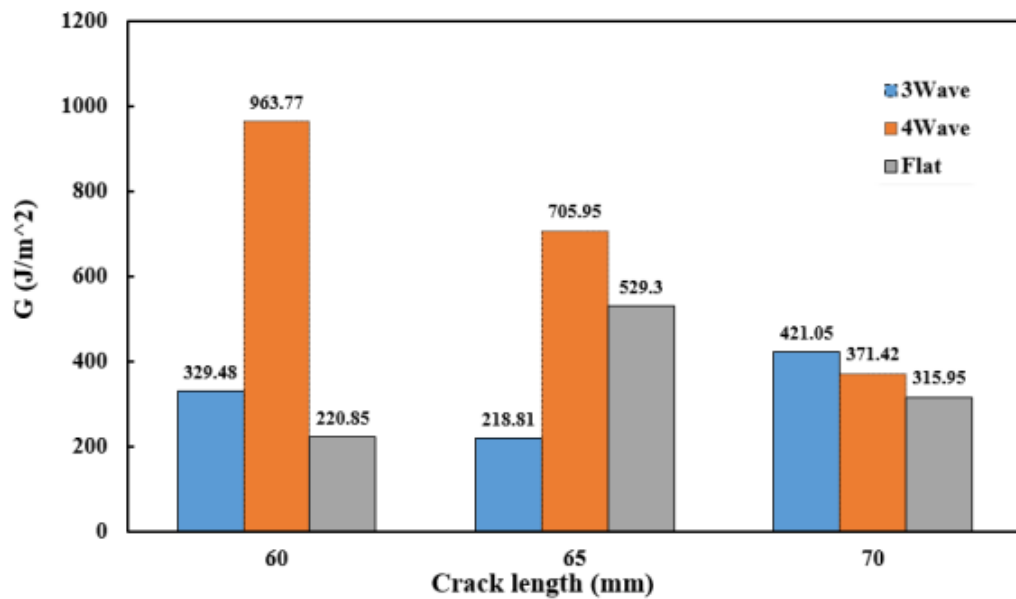
Fig. 3. GI for specimens with different crack length
