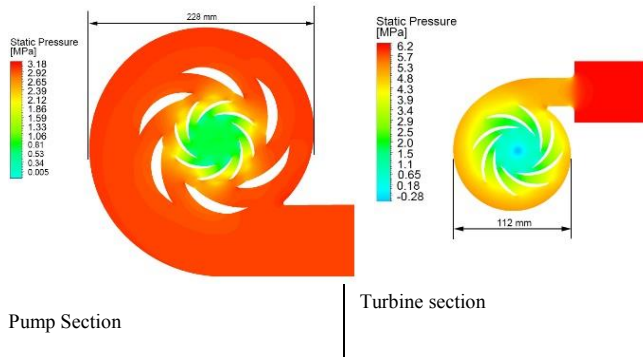
Fig. 2. Static pressure contour in pump and turbine section for new working condition
