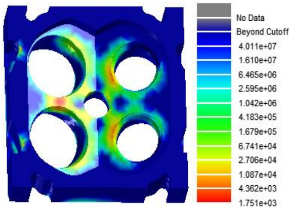
Figure 4. The LCF life prediction in the cylinder head under viscosity stress
