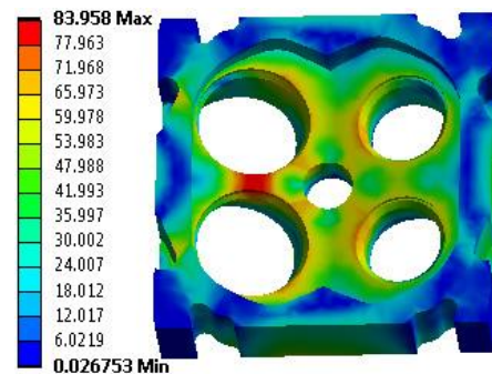
Figure 2. The Von-Mises stress distribution in the cylinder head
