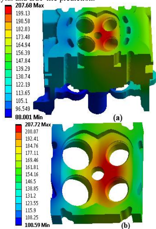
Figure 1. The temperature distribution in the (a) cylinder head and (b) sub-model
