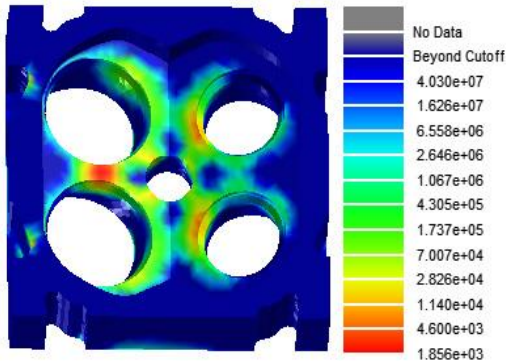
Figure 3. The LCF life prediction in the cylinder head
