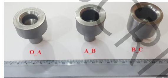
Figure 2. Step-by-step images of the specimens during the extrusion process
