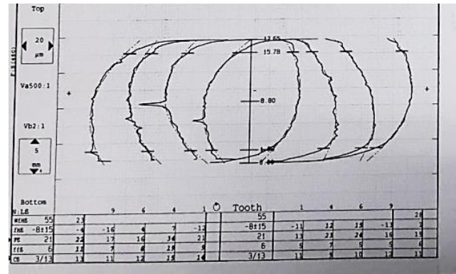
Fig. 6. Laboratory results of gear lead.
