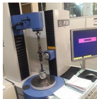
Fig. 4. GMM tooth geometry measuring machine.
