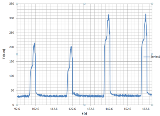
Fig. 5. Test results performed using the device.
