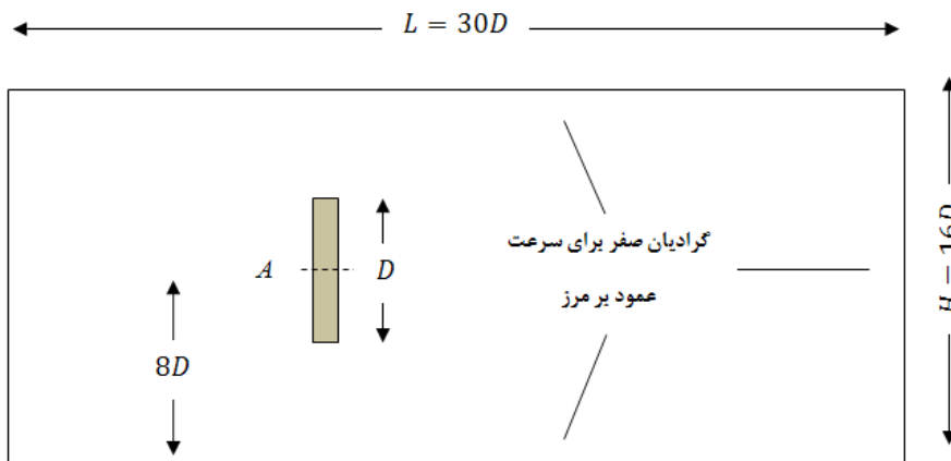
Fig. 3. Schematic of computational domain of flow which pass over a two-dimensional thin plate
