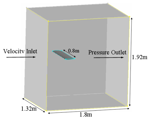
Fig. 10. Geometry of numerical simulation domain and boundary conditions
