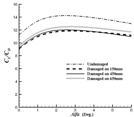
Fig. 20. The lift-to-drag ratio for undamaged and damaged wing in different span positions
