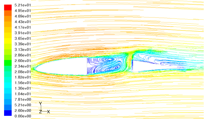
Fig. 16. Numerical result, side view of path lines colored by velocity magnitude on damage center line at 0° angle of attack
