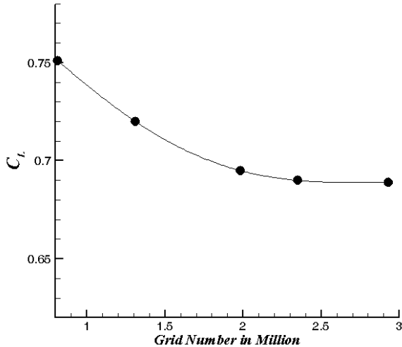
Fig. 7. Grid independency study at 6° angle of attack
