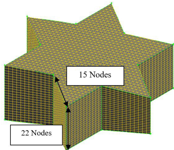
Fig. 9. Quality of the grid inside the damage
