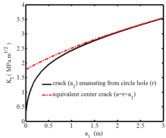
Fig. 3. SIFs for equivalent center crack and cracks emanating from a circular hole
