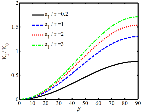
Fig. 7. KI for a circular hole with one crack under loading N_1=1 , N_2=0 and different \beta
