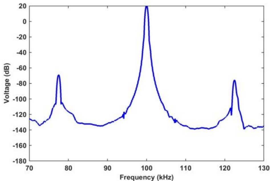
Fig. 3 Spectrum of the structural response to pump (22 kHz) and probe (100 kHz) excitations in the damage state
