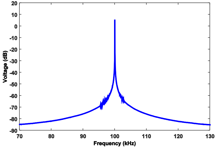
Fig. 2 Spectrum of structural response to pump (22 kHz) and probe (100 kHz) excitations in the healthy state
