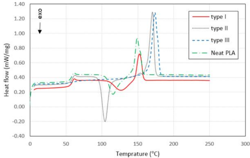
Fig. 2. The DSC thermograms of the second heating cycle for three different PLA filament brands and neat PLA.
