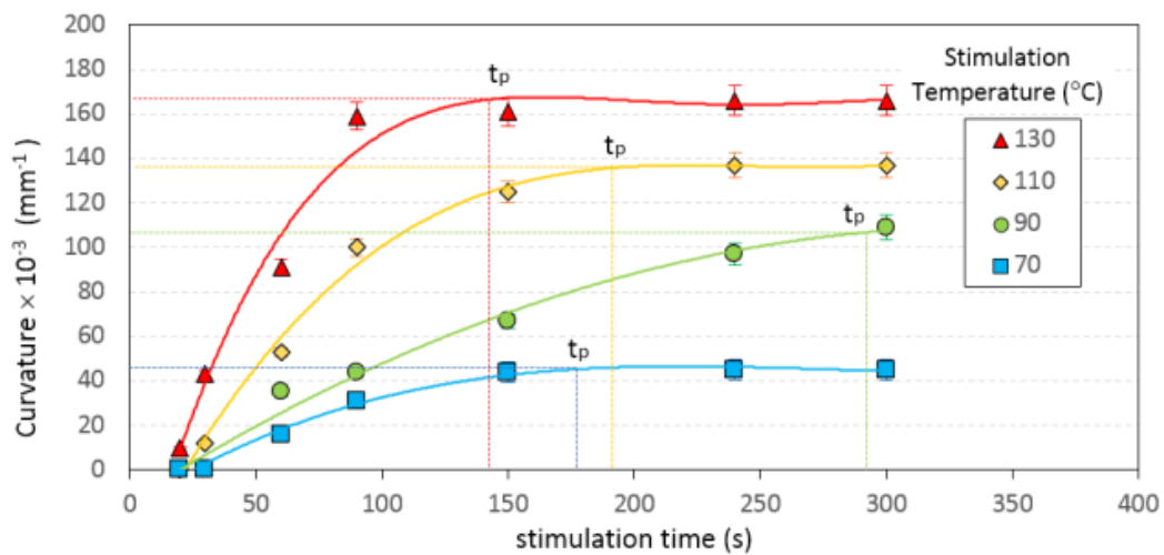
Fig. 3. The effects of the activation parameters on the resulting curvature.
