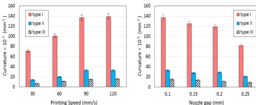
Fig. 1. The effects of the manufacturing and material parameters on the resulting curvature.
