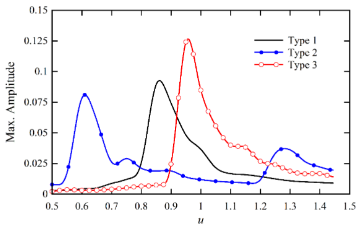
Fig. 5. The maximum amplitude of vibration of a viscoelastic beam's midpoint in terms of external fluid flow velocity
