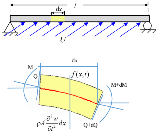
Fig. 2. Simply supported viscoelastic beam under the influence of external fluid and a section of the beam
