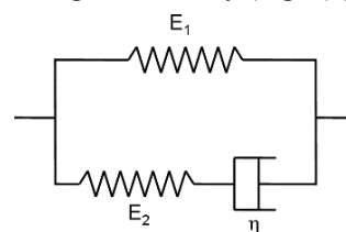
Fig. 1. Standard Linear Solid model
