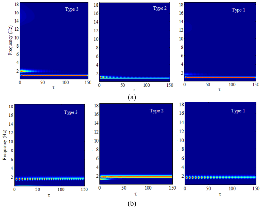
Fig. 4. Wavelet transform of viscoelastic beam for different fluid flow velocity a) u = 0.5 b) u = 1
