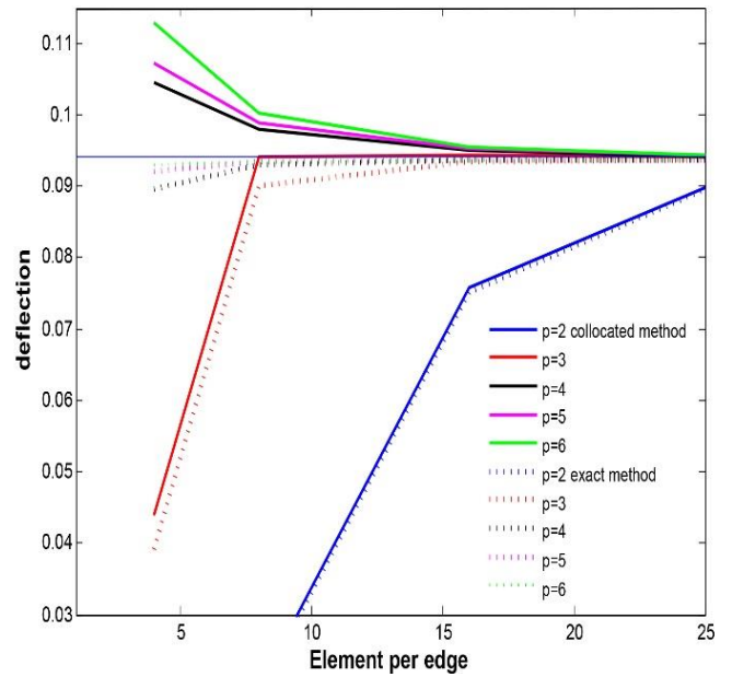
Fig 2. Comparison of deformation convergence behavior of hemispherical shell for various order of the NURBS
