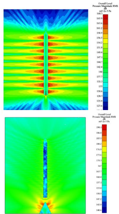
Fig. 4. a) Vertical interface of the projectile without jet flow deflector, and b) vertical interface of the projectile with a jet flow deflector.
