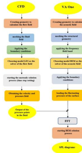
Fig. 1. Schematic flowchart of hybrid CFD/BEM approach
