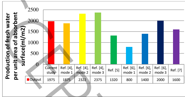
Figure 1: Comparison of the maximum production of fresh water per unit area of absorbent surface
