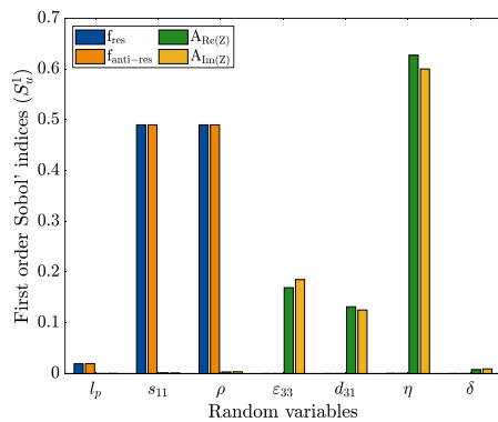
Figure 1. First order Sobol' sensitivity indices for RVs
